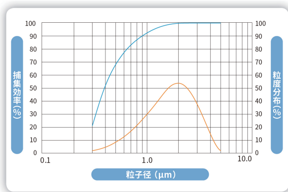
MJ-15CS捕集效率
